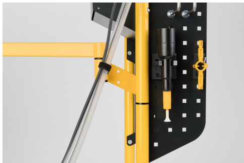
Multifunctional head module of the manual system with storage areas and hanging options for tools and accessories
